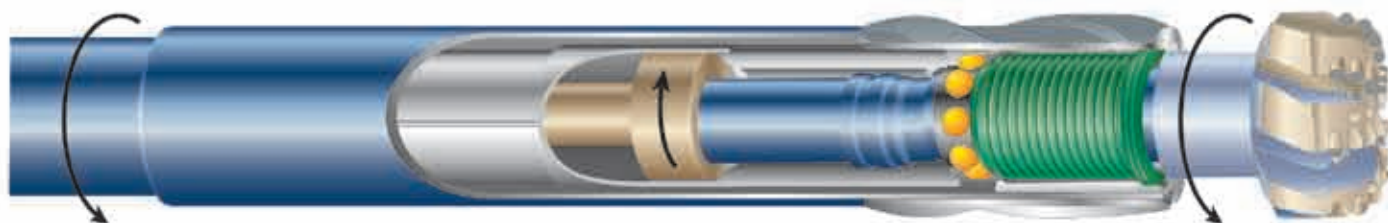
Figure 1 - At the heart of the fully rotating technology is a continuously rotating internal cam that changed the angle of the drive shaft, keeping the bit pointed in the desired direction at all times.
