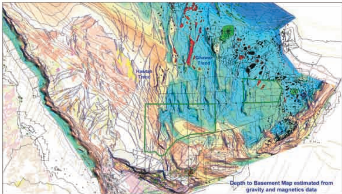
Figure 3 - Plate-wide depth to basement map based on potential field data.
