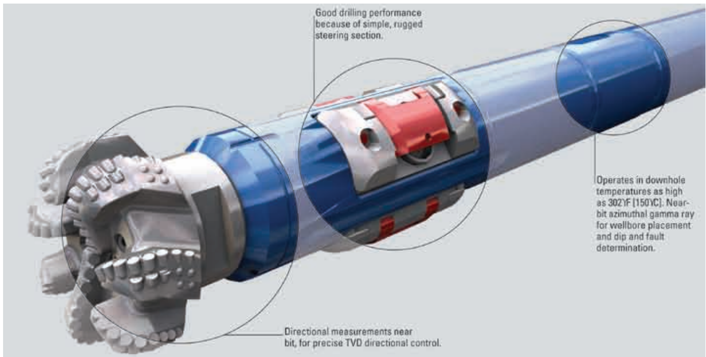
Figure 2 - PowerDrive X5*.
