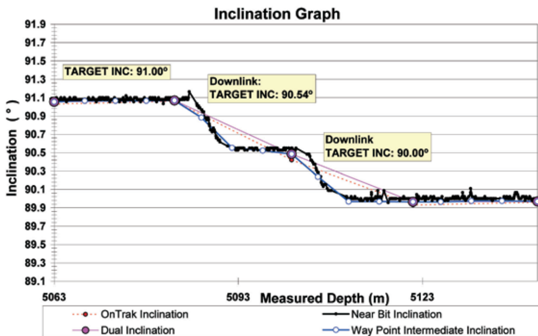
Figure 2 - The black curve shows "Near Bit Inclination" (NBI) data which is measured and reported continuously close to the bit at high speed. Inclination provided by the directional survey sensors (red curve) is subsequently combined with this NBI data (blue curve) using proprietary Survey Management algorithms to provide a more accurate definition of the wellbores vertical position and its associated uncertainties.
