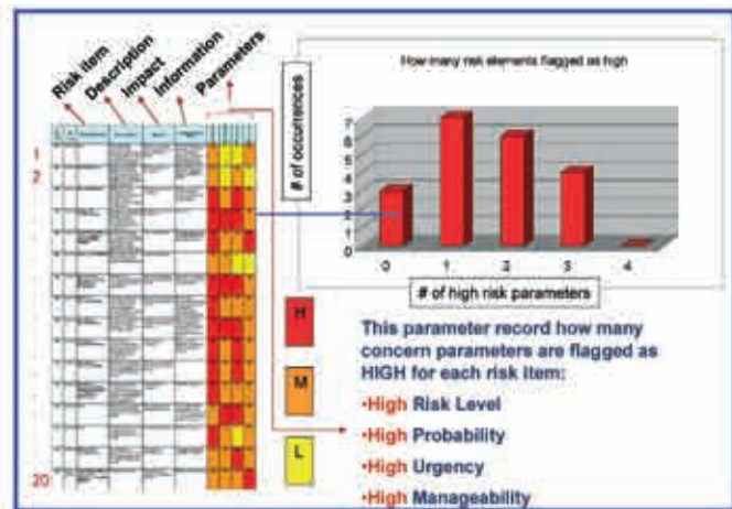
Figure 9 - Risk analysis.
